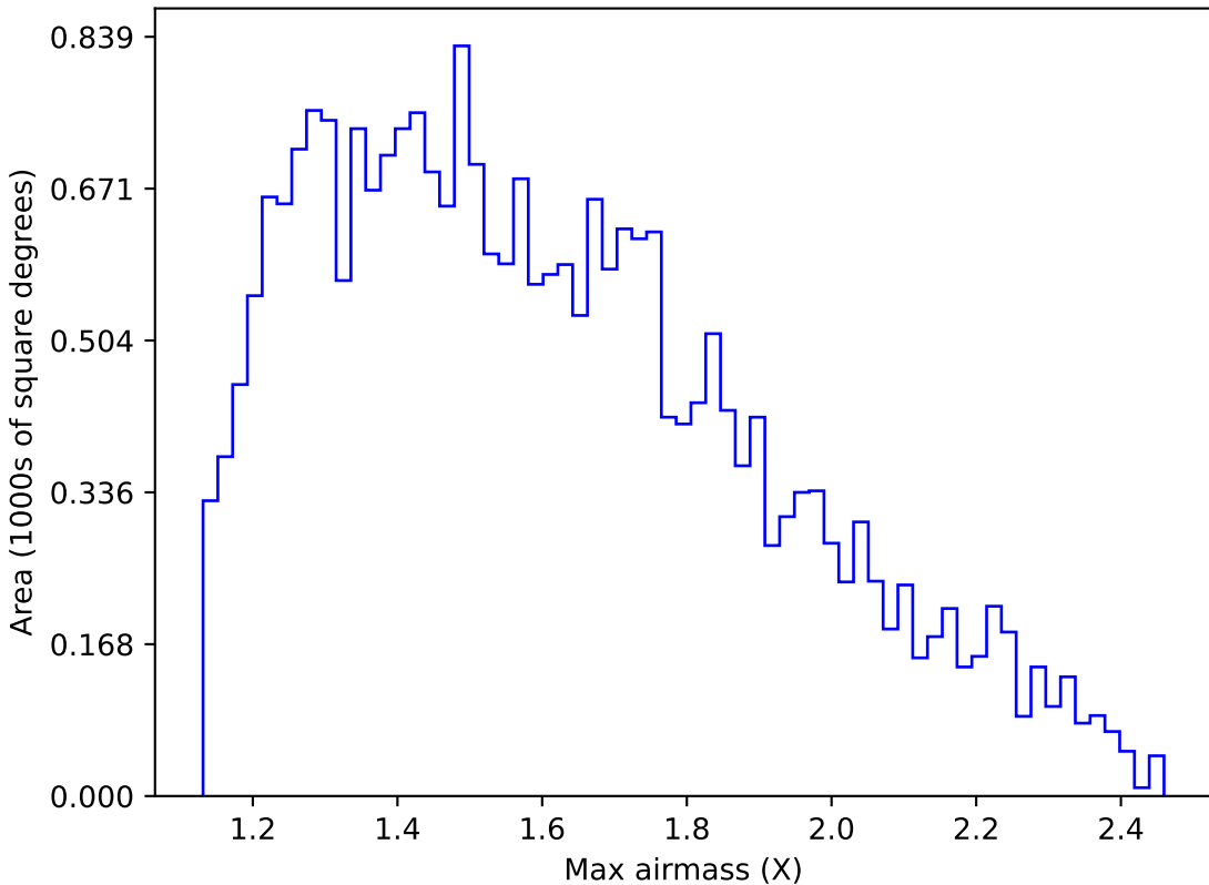
weather_cloudso35v3.4_10yrs Yr 1 g band: Max airmass
