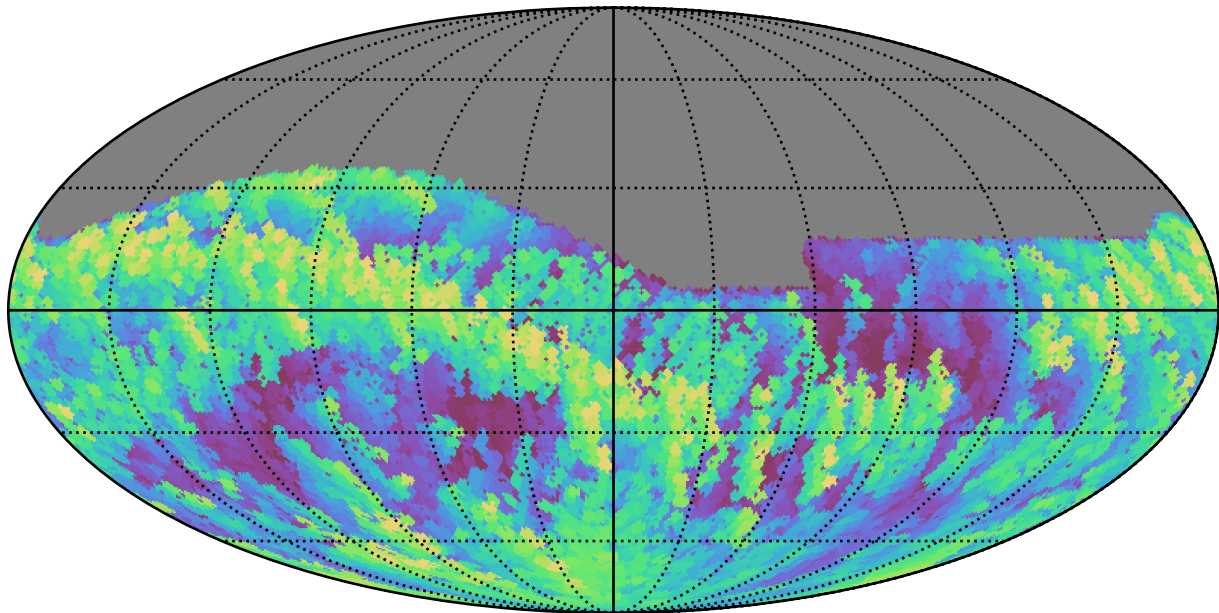
weather_cloudso35v3.4_10yrs Yr 1 all bands: Max airmass
