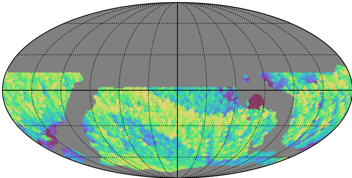
weather_cloudso35v3.4_10yrs WFD z band: Max airmass
