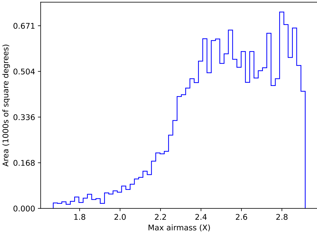
weather_cloudso35v3.4_10yrs WFD z band: Max airmass
