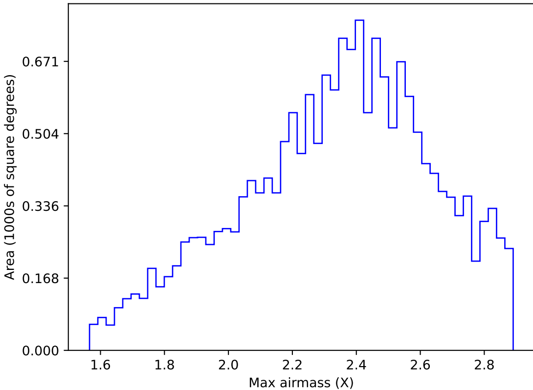
weather_cloudso35v3.4_10yrs WFD y band: Max airmass
