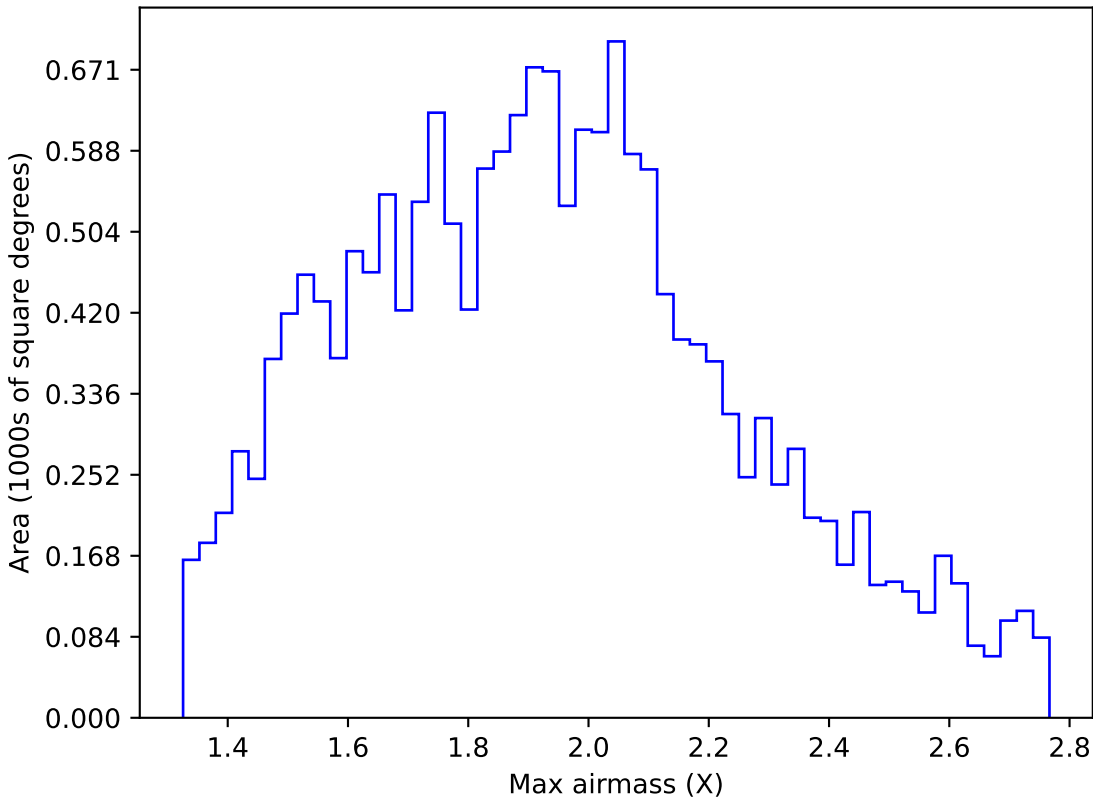
weather_cloudso35v3.4_10yrs WFD u band: Max airmass
