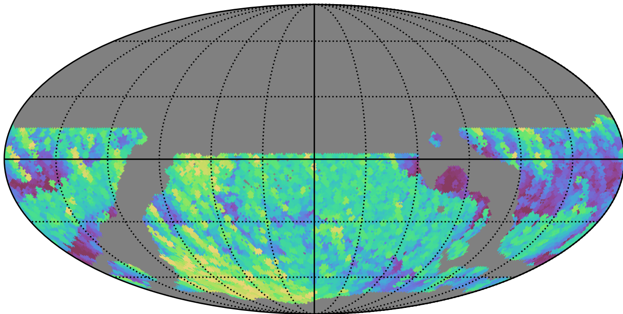
weather_cloudso35v3.4_10yrs WFD r band: Max airmass
