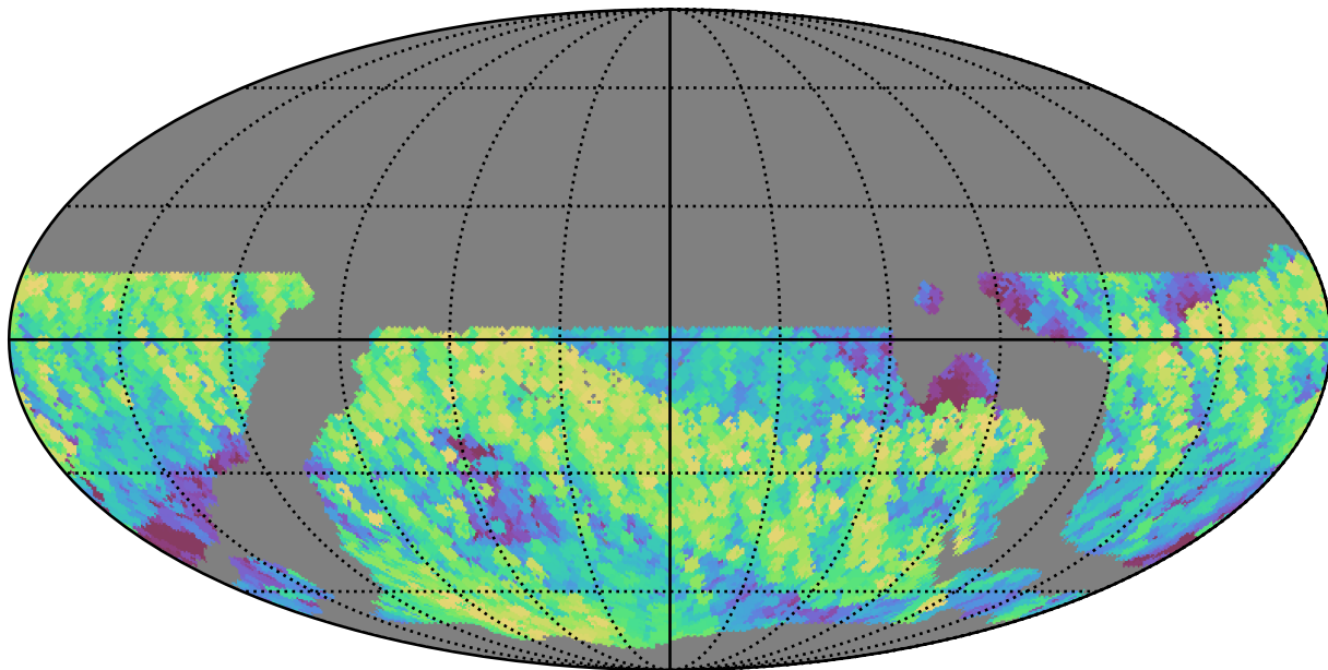
weather_cloudso35v3.4_10yrs WFD i band: Max airmass
