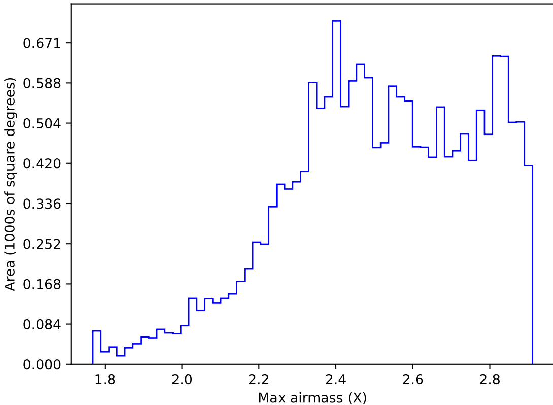
weather_cloudso35v3.4_10yrs WFD i band: Max airmass
