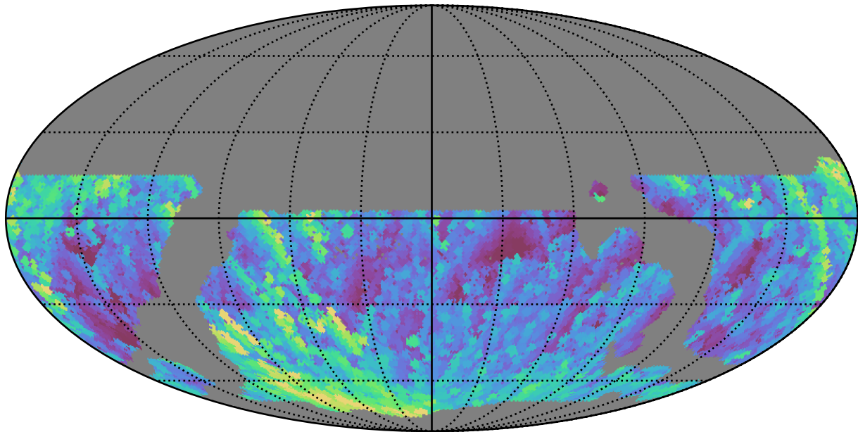
weather_cloudso35v3.4_10yrs WFD g band: Max airmass
