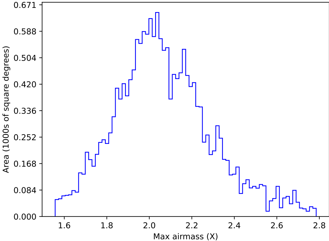
weather_cloudso35v3.4_10yrs WFD g band: Max airmass
