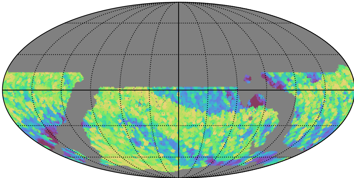
weather_cloudso35v3.4_10yrs WFD all bands: Max airmass
