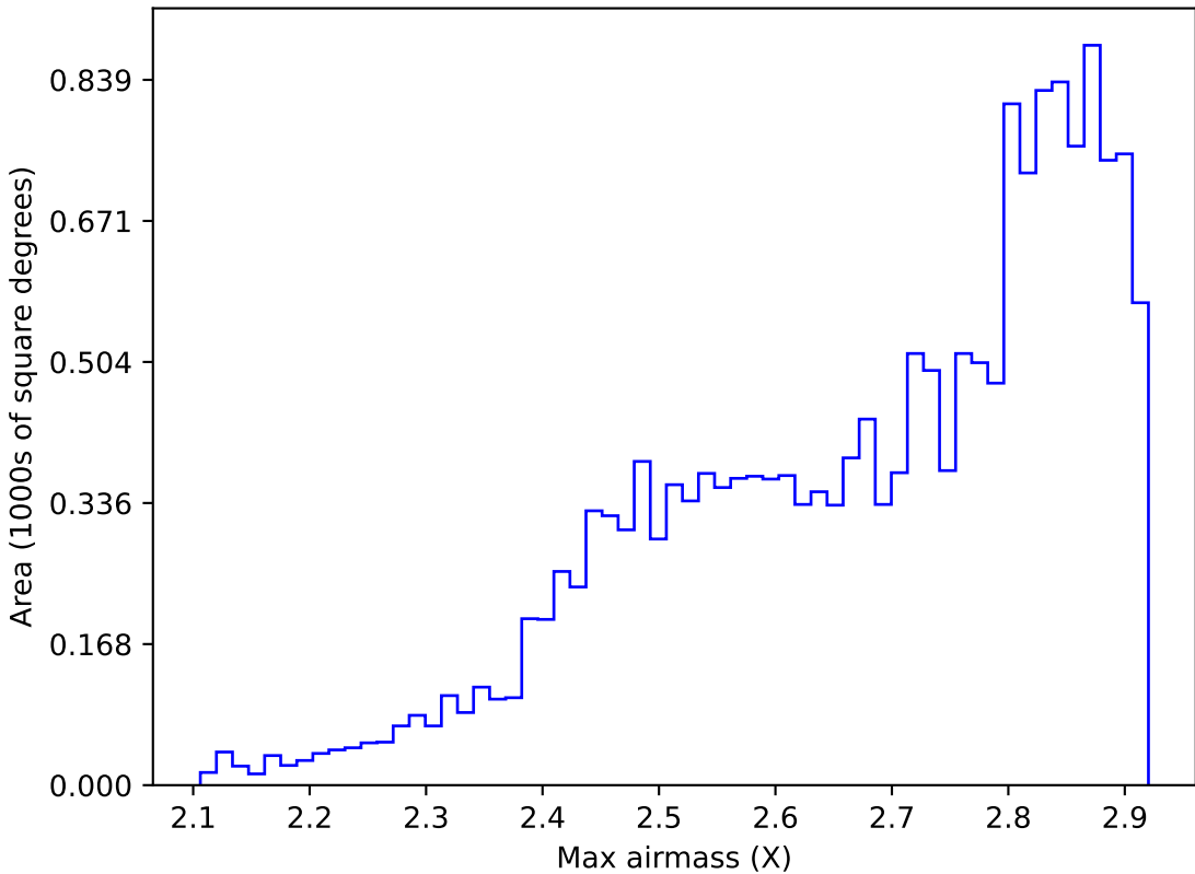
weather_cloudso35v3.4_10yrs WFD all bands: Max airmass
