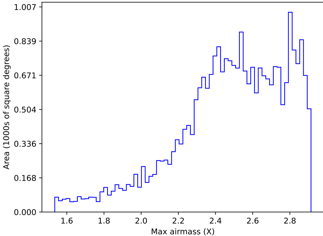
weather_cloudso35v3.4_10yrs All sky z band: Max airmass
