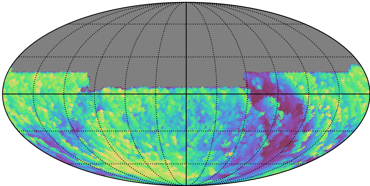
weather_cloudso35v3.4_10yrs All sky y band: Max airmass
