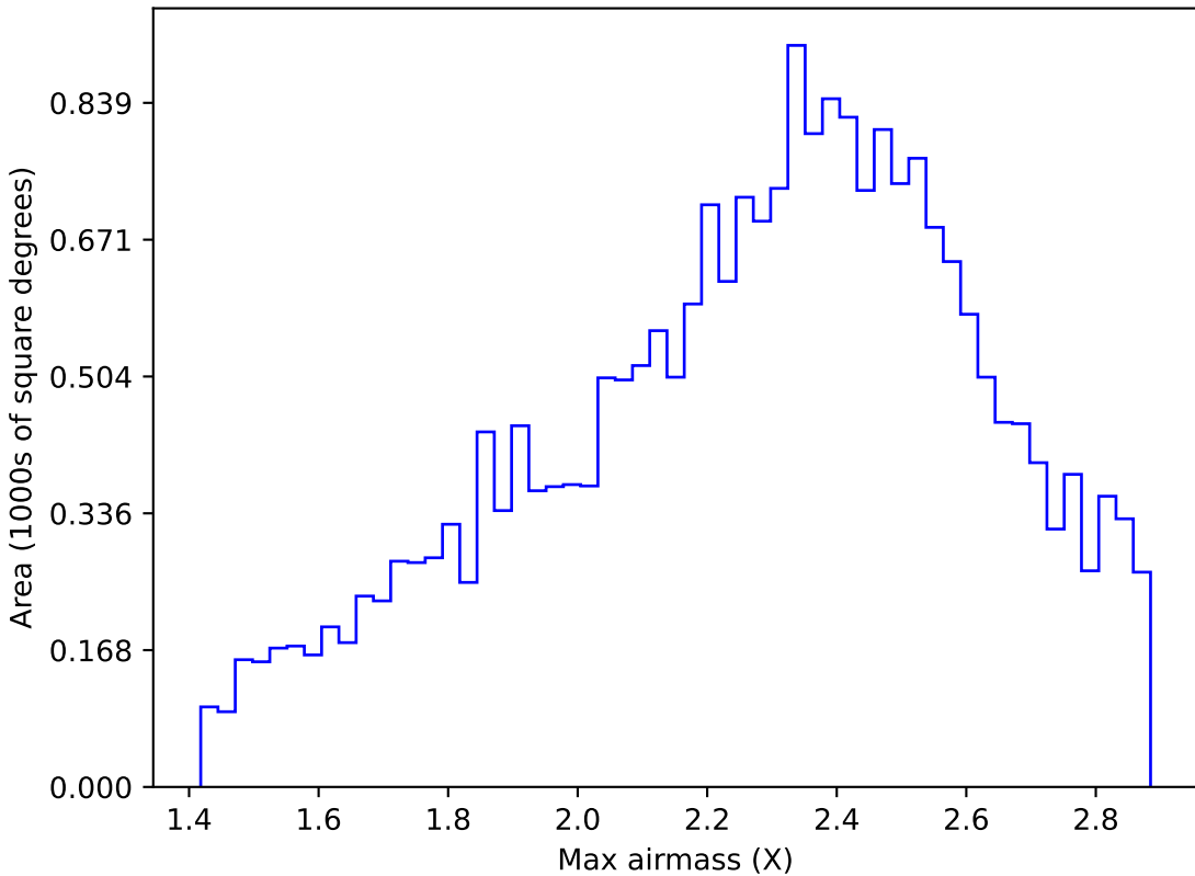
weather_cloudso35v3.4_10yrs All sky y band: Max airmass
