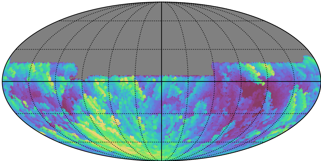
weather_cloudso35v3.4_10yrs All sky u band: Max airmass
