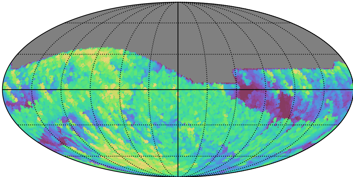
weather_cloudso35v3.4_10yrs All sky r band: Max airmass
