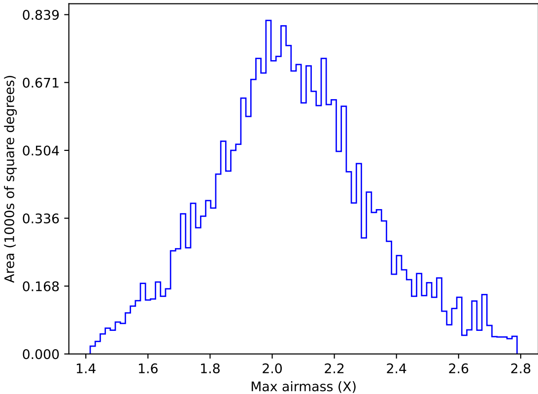
weather_cloudso35v3.4_10yrs All sky g band: Max airmass
