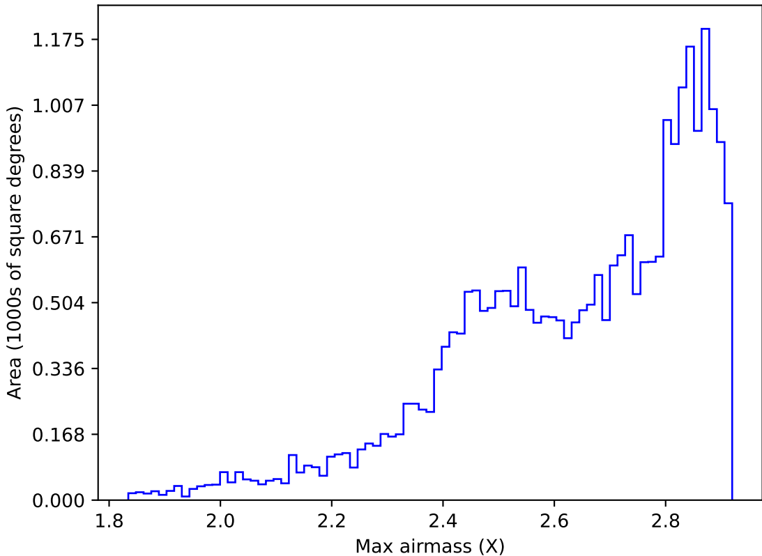
weather_cloudso35v3.4_10yrs All sky all bands: Max airmass
