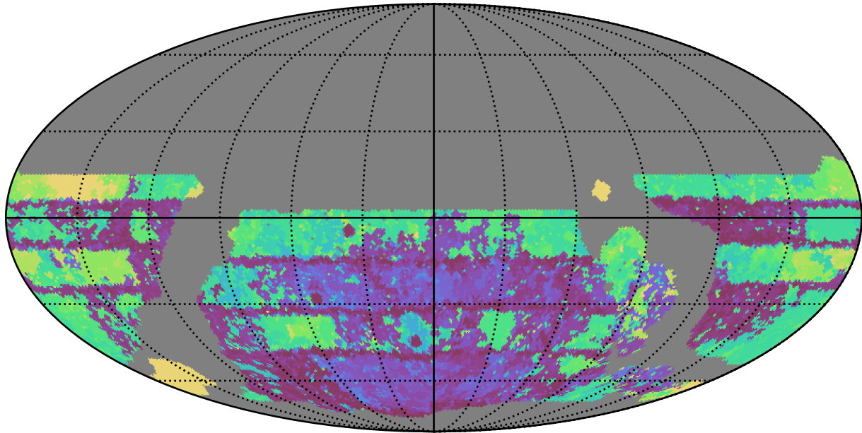
weather_cloudso35v3.4_10yrs WFD u band: Max Inter-Night Gap
