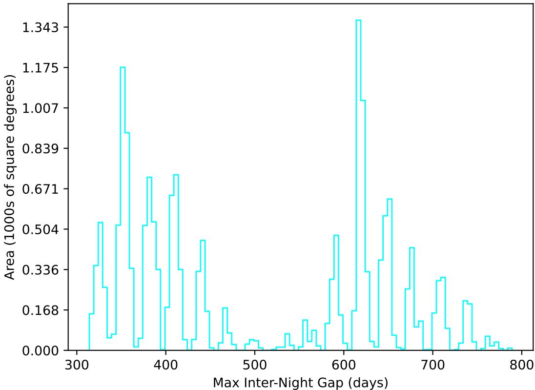
weather_cloudso35v3.4_10yrs WFD u band: Max Inter-Night Gap
