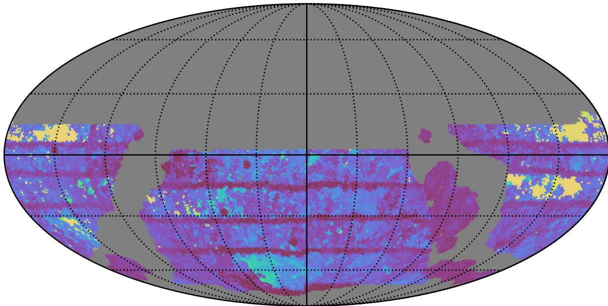
weather_cloudso35v3.4_10yrs WFD r band: Max Inter-Night Gap
