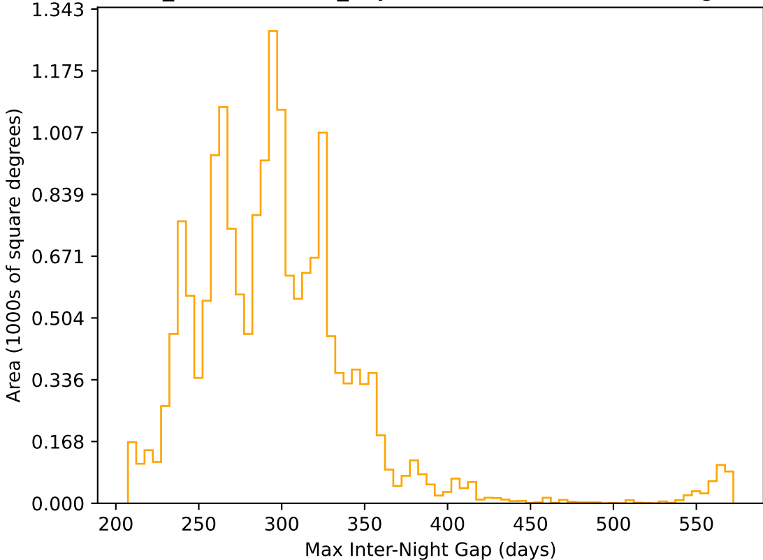
weather_cloudso35v3.4_10yrs WFD r band: Max Inter-Night Gap
