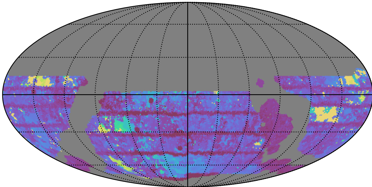
weather_cloudso35v3.4_10yrs WFD i band: Max Inter-Night Gap
