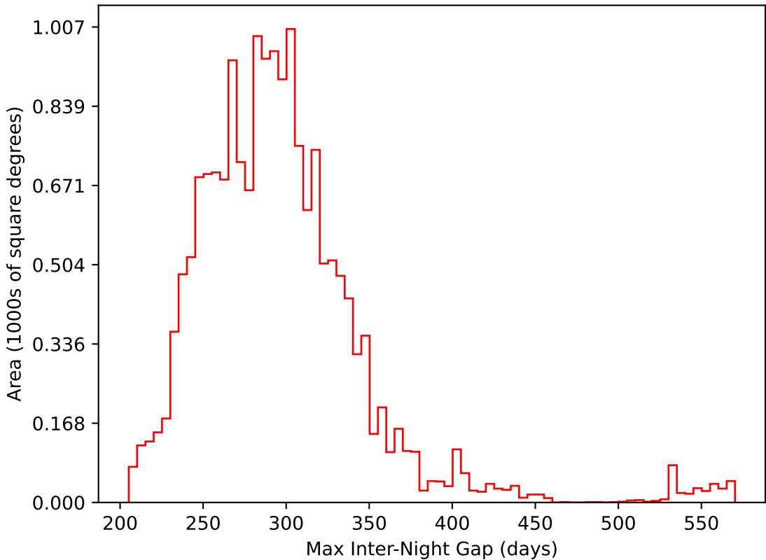
weather_cloudso35v3.4_10yrs WFD i band: Max Inter-Night Gap
