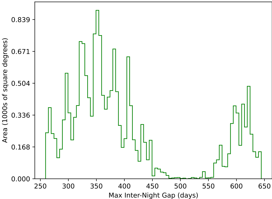
weather_cloudso35v3.4_10yrs WFD g band: Max Inter-Night Gap
