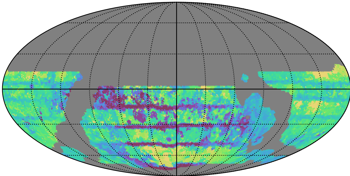
weather_cloudso35v3.4_10yrs WFD all bands: Max Inter-Night Gap
