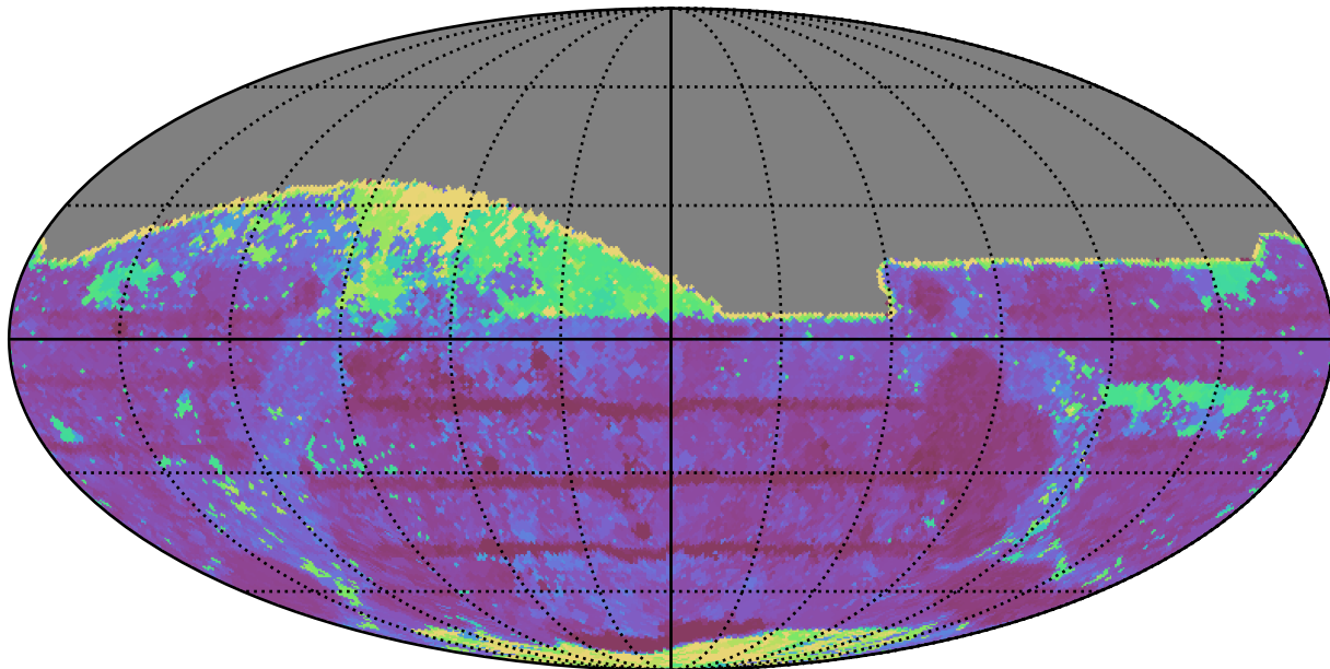
weather_cloudso35v3.4_10yrs All sky z band: Max Inter-Night Gap
