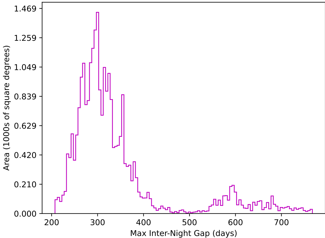
weather_cloudso35v3.4_10yrs All sky z band: Max Inter-Night Gap
