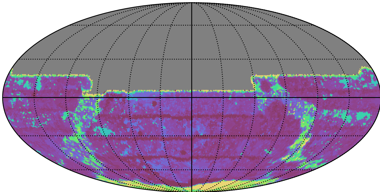
weather_cloudso35v3.4_10yrs All sky y band: Max Inter-Night Gap
