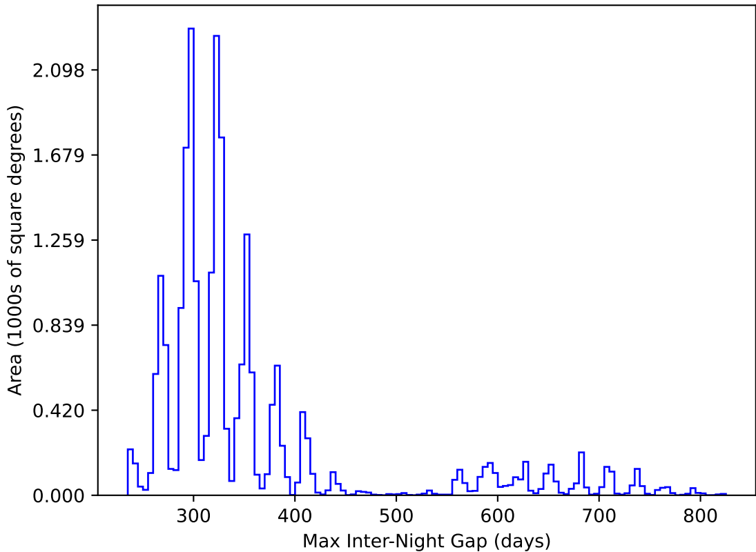
weather_cloudso35v3.4_10yrs All sky y band: Max Inter-Night Gap
