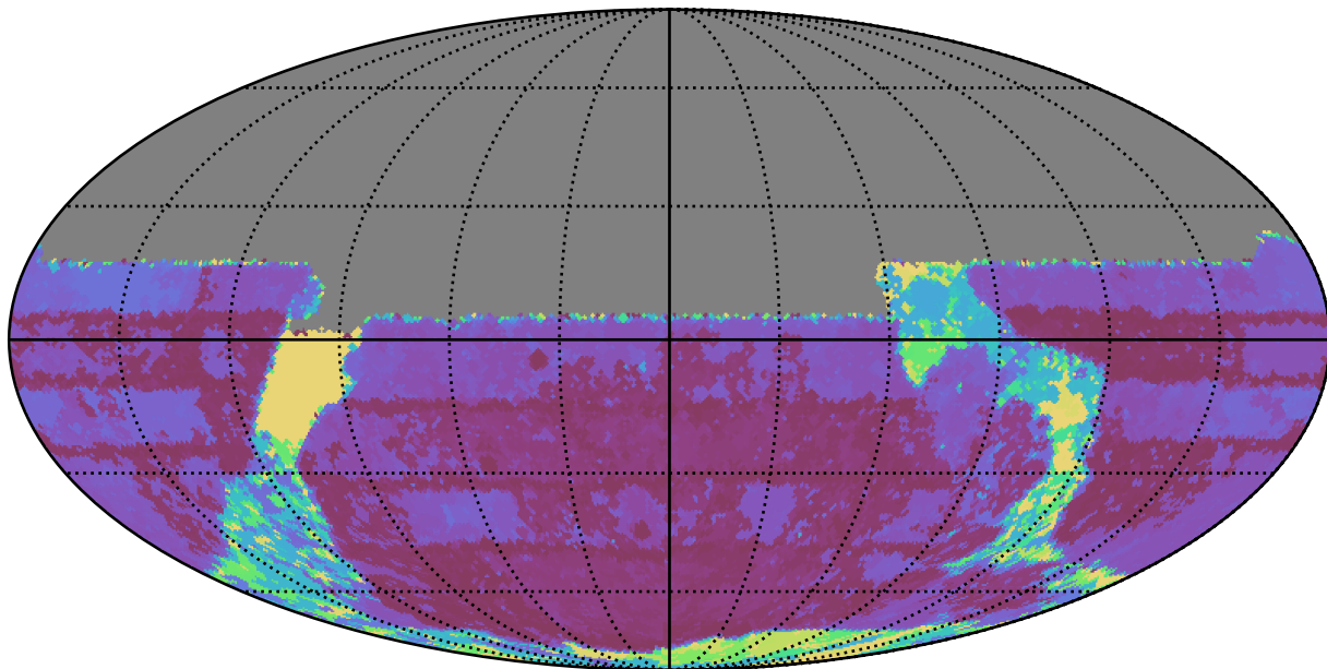
weather_cloudso35v3.4_10yrs All sky u band: Max Inter-Night Gap
