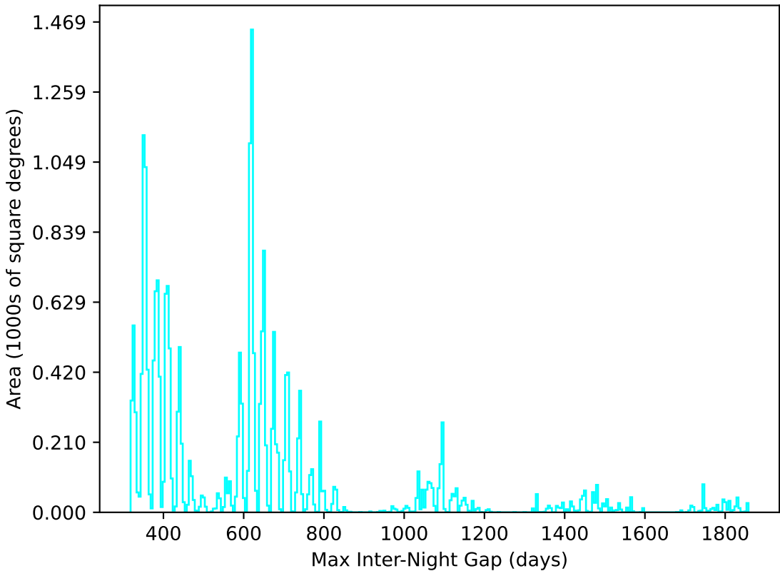
weather_cloudso35v3.4_10yrs All sky u band: Max Inter-Night Gap
