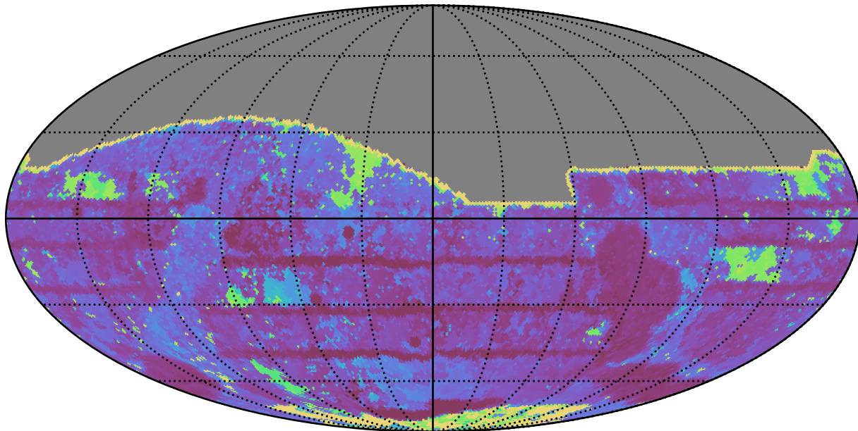
weather_cloudso35v3.4_10yrs All sky i band: Max Inter-Night Gap
