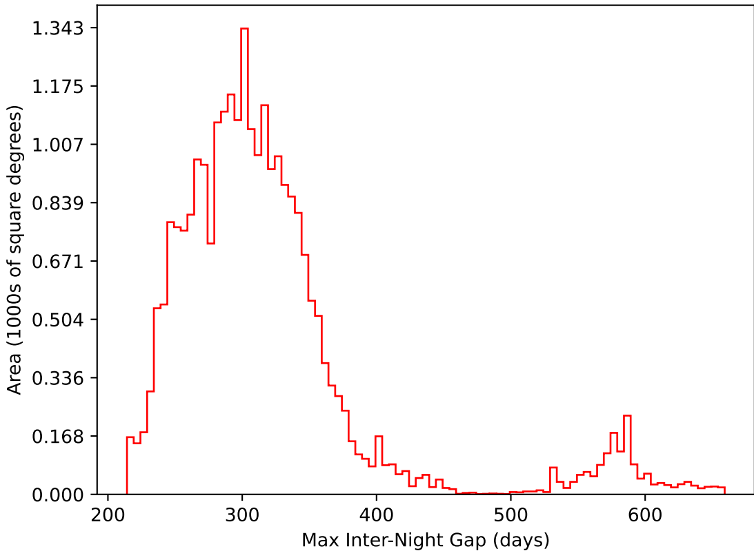
weather_cloudso35v3.4_10yrs All sky i band: Max Inter-Night Gap
