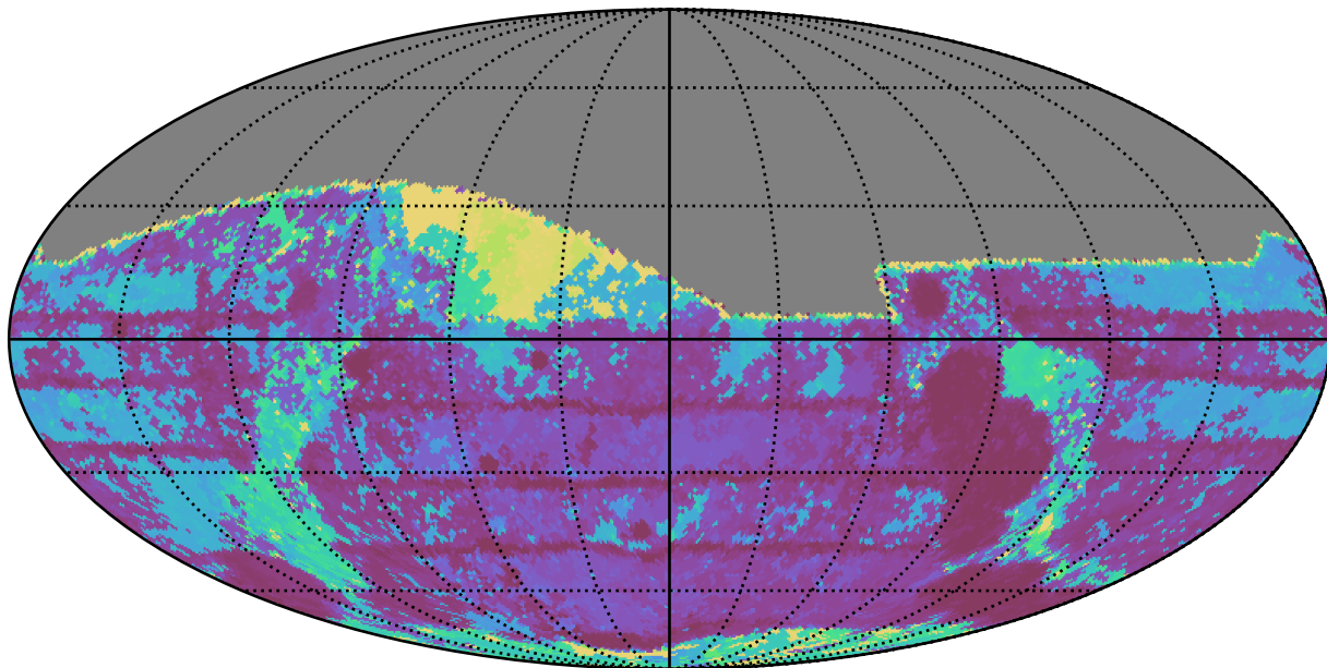
weather_cloudso35v3.4_10yrs All sky g band: Max Inter-Night Gap
