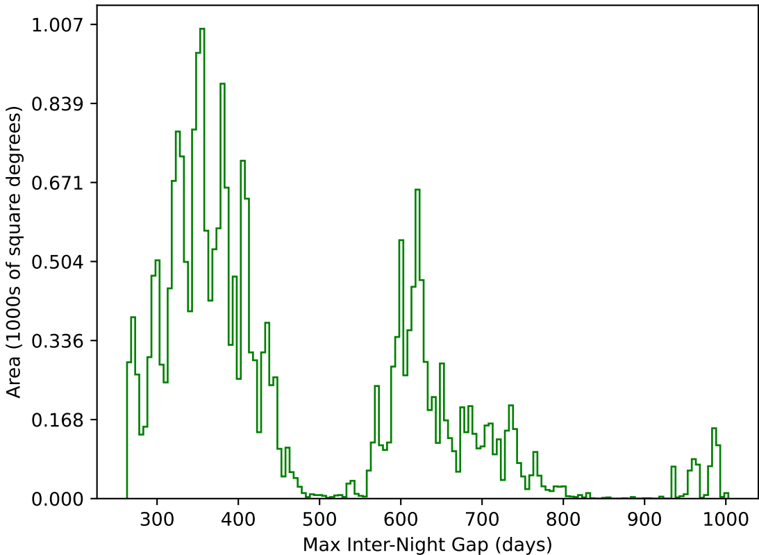
weather_cloudso35v3.4_10yrs All sky g band: Max Inter-Night Gap
