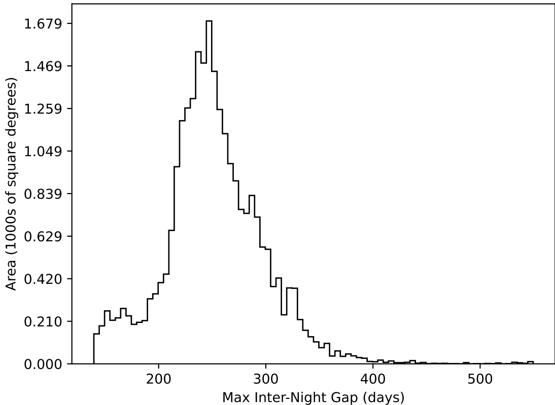
weather_cloudso35v3.4_10yrs All sky all bands: Max Inter-Night Gap
