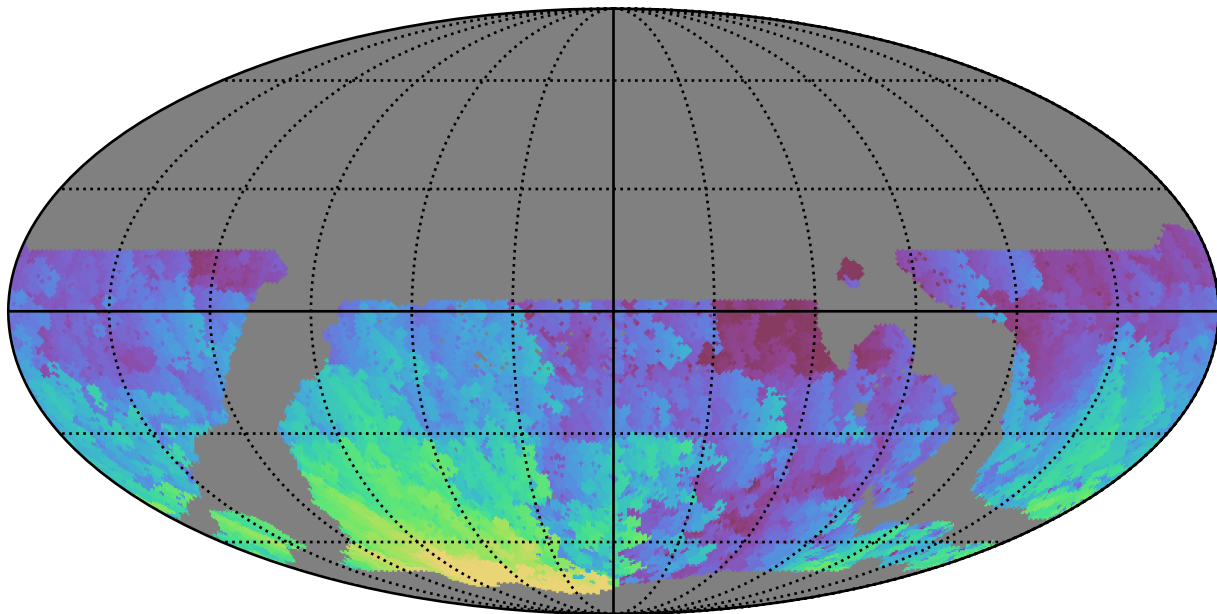
weather_cloudso35v3.4_10yrs WFD u band: Max HA
