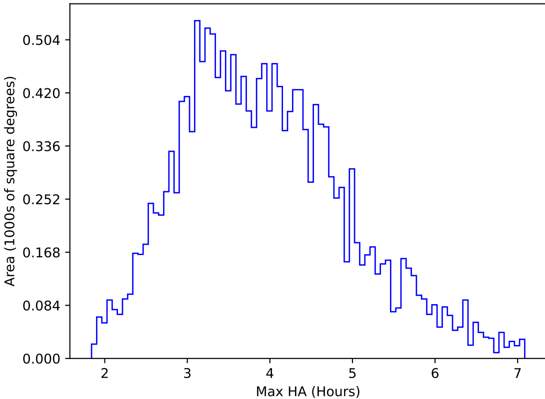
weather_cloudso35v3.4_10yrs WFD u band: Max HA
