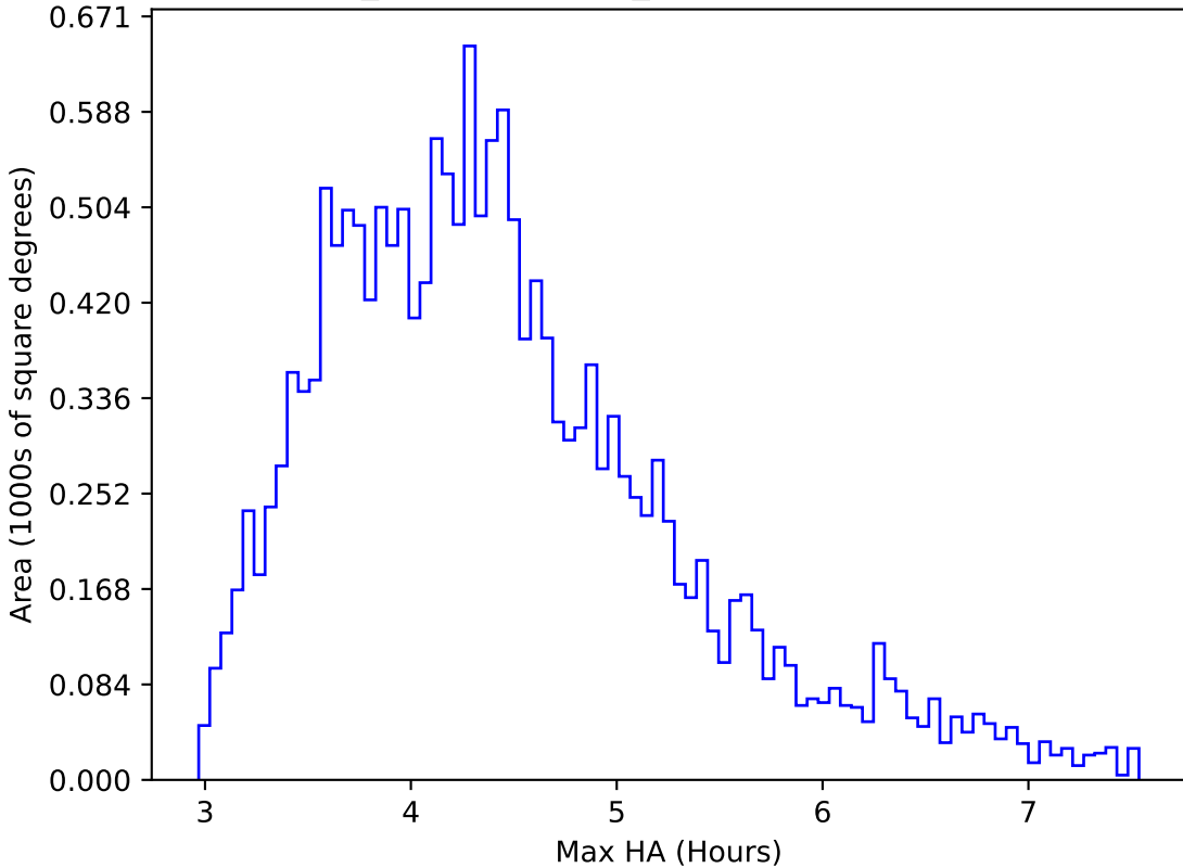
weather_cloudso35v3.4_10yrs WFD r band: Max HA
