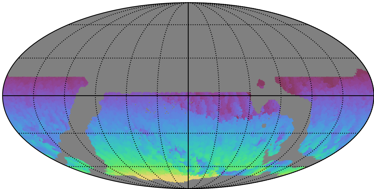
weather_cloudso35v3.4_10yrs WFD all bands: Max HA
