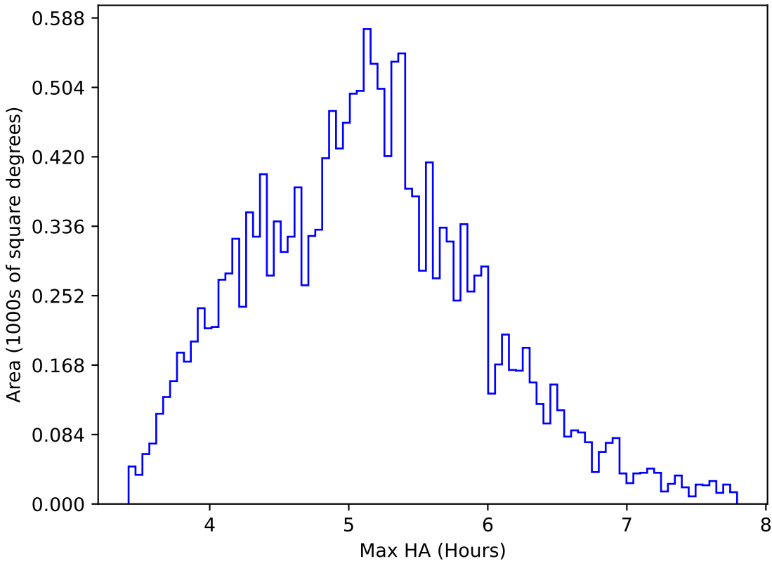
weather_cloudso35v3.4_10yrs WFD all bands: Max HA
