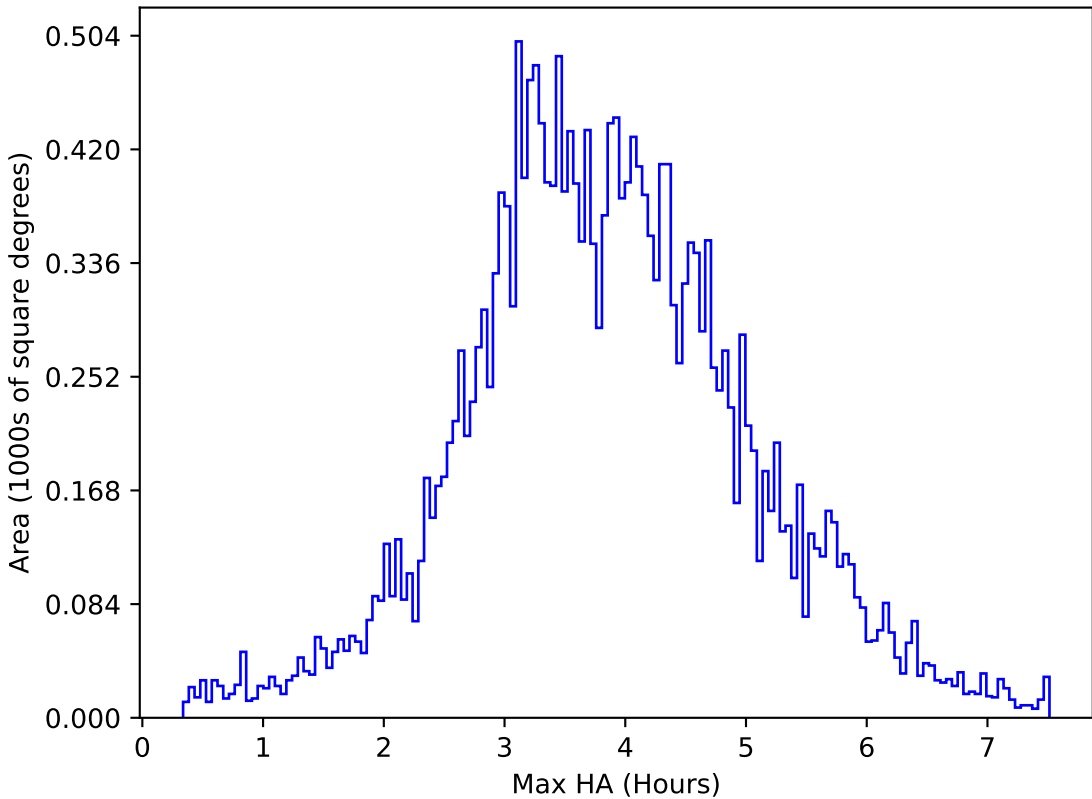
weather_cloudso35v3.4_10yrs All sky u band: Max HA
