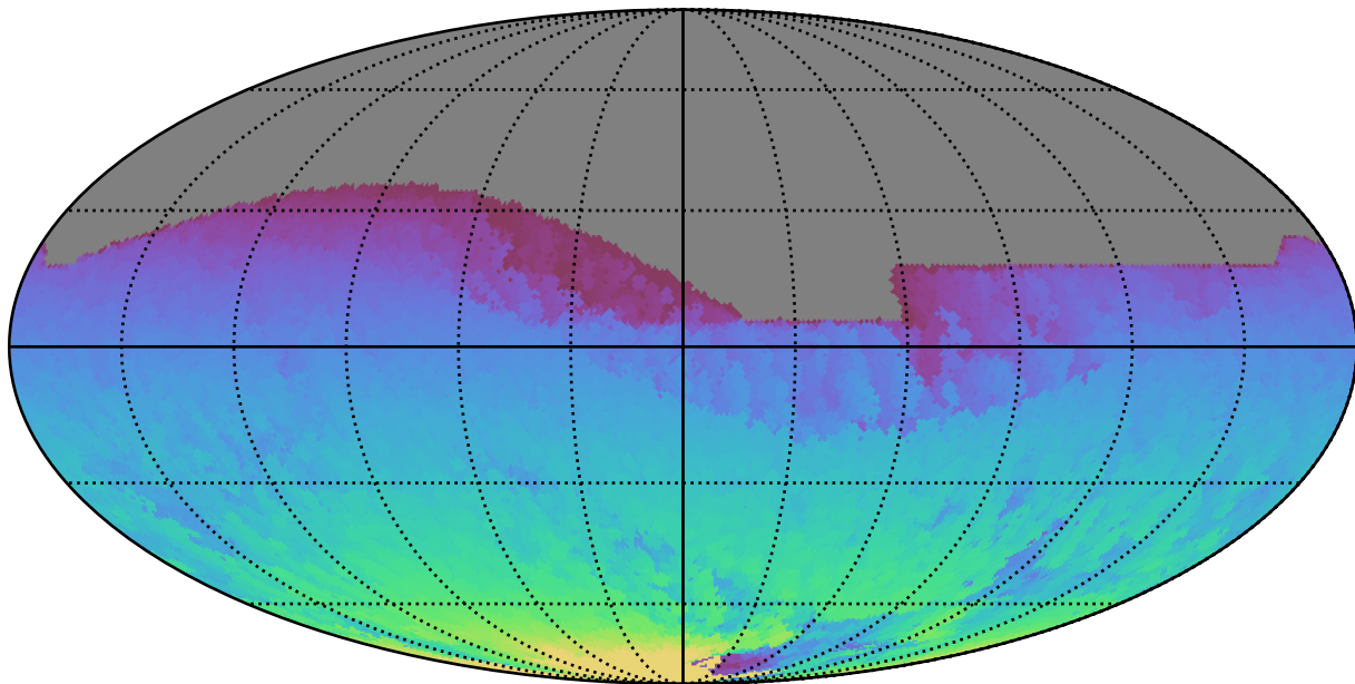
weather_cloudso35v3.4_10yrs All sky all bands: Max HA
