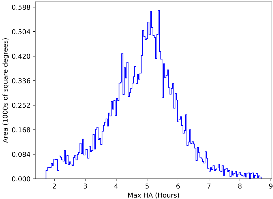
weather_cloudso35v3.4_10yrs All sky all bands: Max HA
