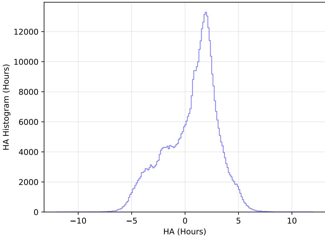
weather_cloudso35v3.4_10yrs WFD z band: HA Histogram
