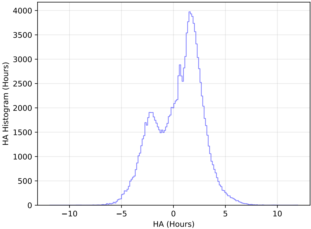
weather_cloudso35v3.4_10yrs WFD u band: HA Histogram
