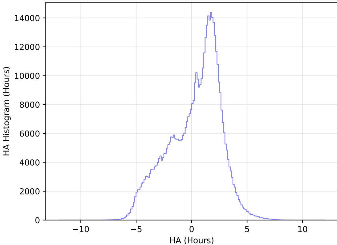
weather_cloudso35v3.4_10yrs WFD r band: HA Histogram
